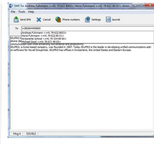
SkySMS Client
