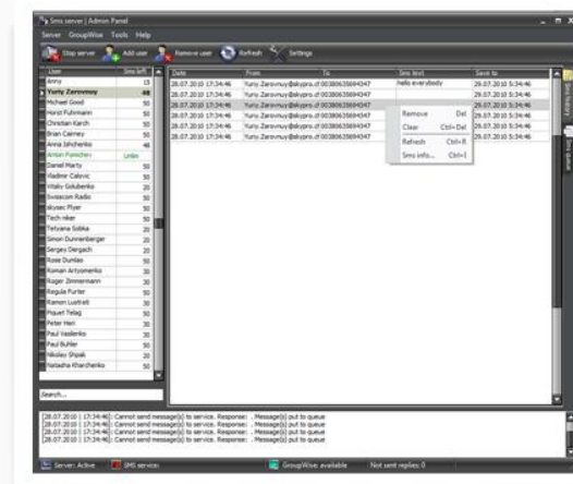
SkySMS Server
