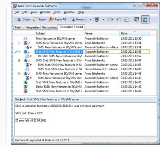
SMS Thread
