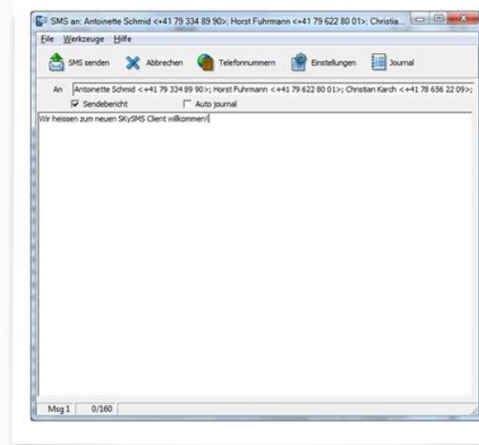
SKySMS Client
